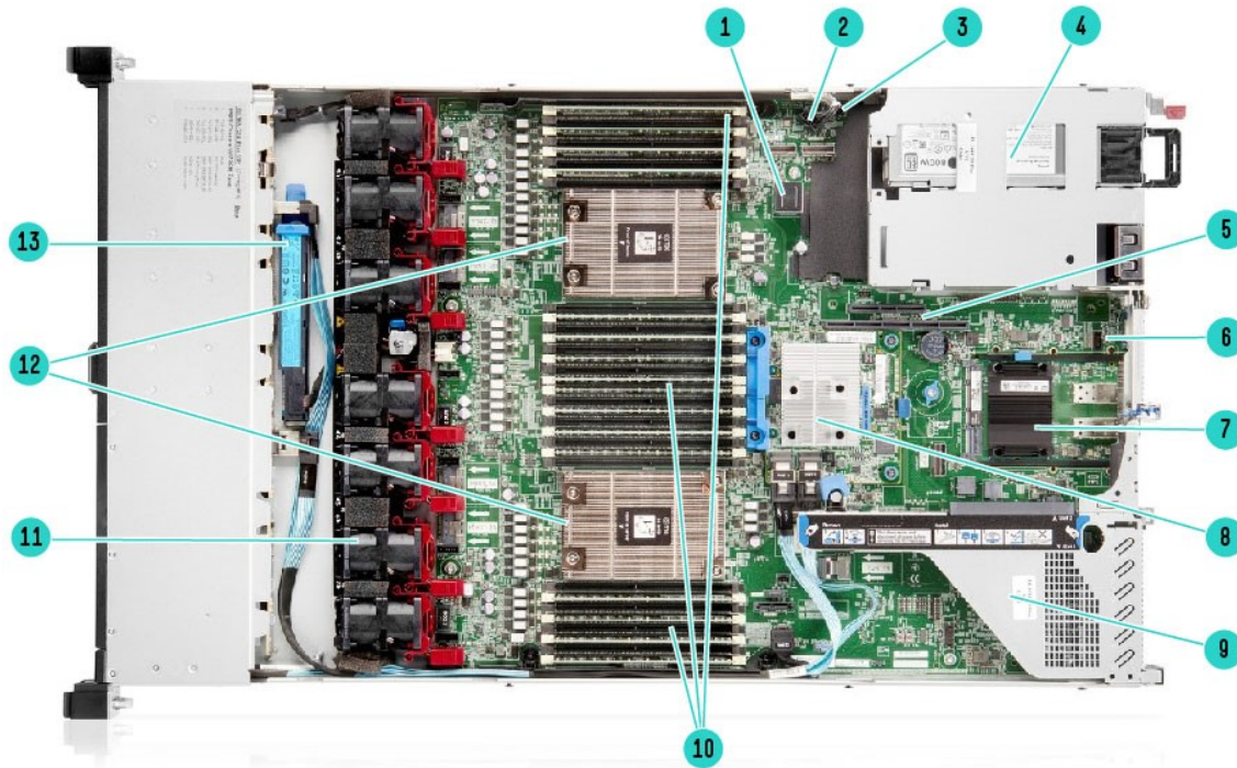
Internal View - Standard for all DL365 Gen10 Plus
